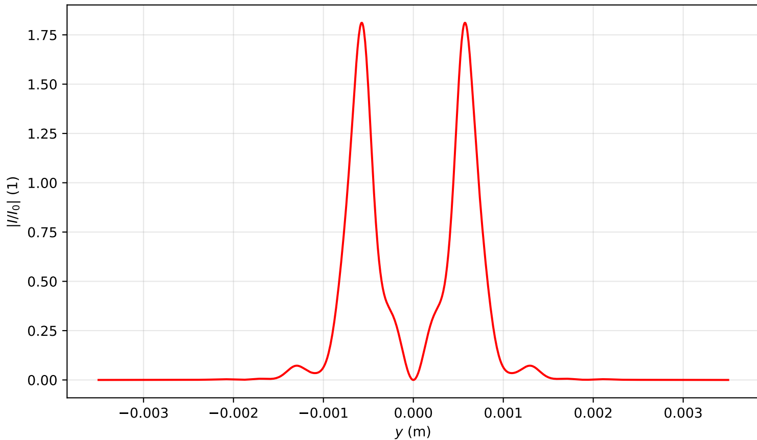
Intensity profile I(x=0, y, z=1.194)/I_0 , P_{in}=8.0P_{cr} , artificial time
